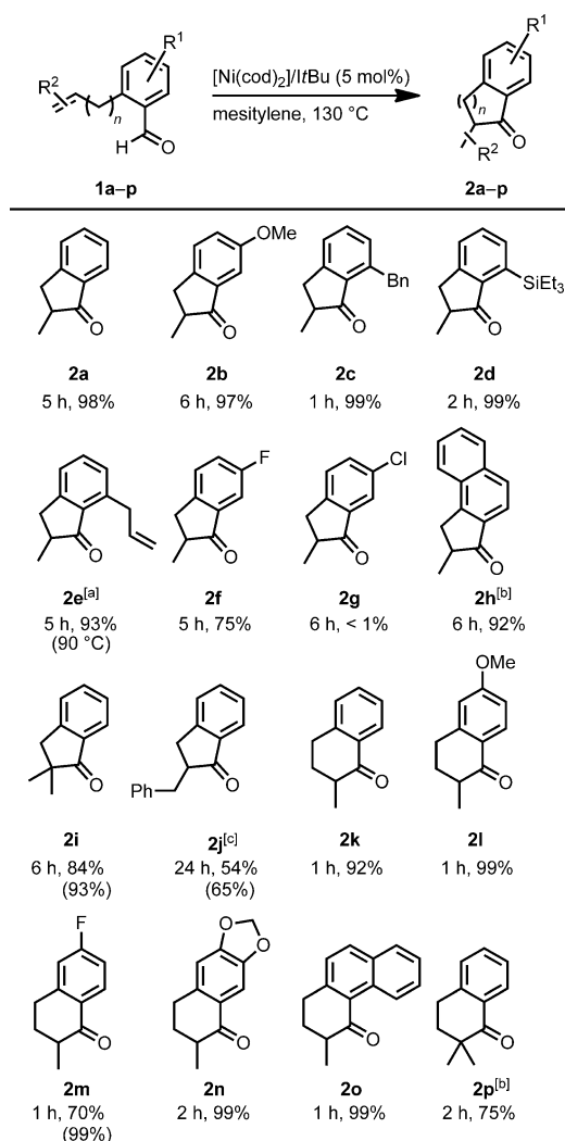
Scheme 3. Ni 0 -catalyzed intramolecular alkene hydroacylation. Reaction conditions: Enal 1a–p (0.80 mmol), [Ni(cod) 2 ]/ It Bu (5 mol %, 0.040 mmol) and mesitylene (2 mL) were reacted at 130 °C. Yields presented are of isolated product; yields determined by GC analysis using n -pentadecane as an internal standard are given in parentheses. [a] [Ni(cod) 2 ] (7 mol %) and It Bu (5 mol %) in toluene were used. [b] [Ni(cod) 2 ]/ It Bu (10 mol %) was used. [c] [Ni(cod) 2 ]/IMes (10 mol %) was used. cod = 1,5-cyclooctadiene. (For the structures of It Bu and IMes, see the Supporting Information).
