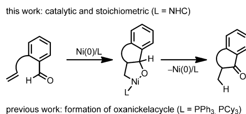
Scheme 2. Catalytic generation of a benzocyclic ketone without decarbonylation.
