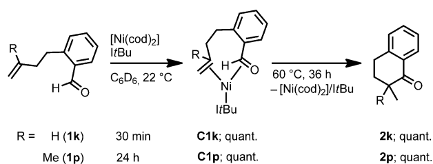
Scheme 5. Stoichiometric reactions with 1k and 1p .
